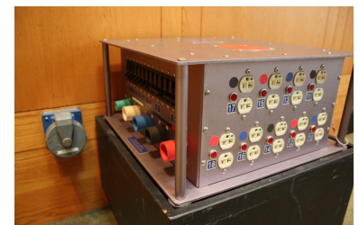
Distro Box w/ Pin & Sleeve plug
