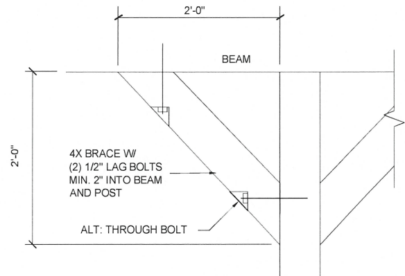
KNEE BRACE DETAIL
